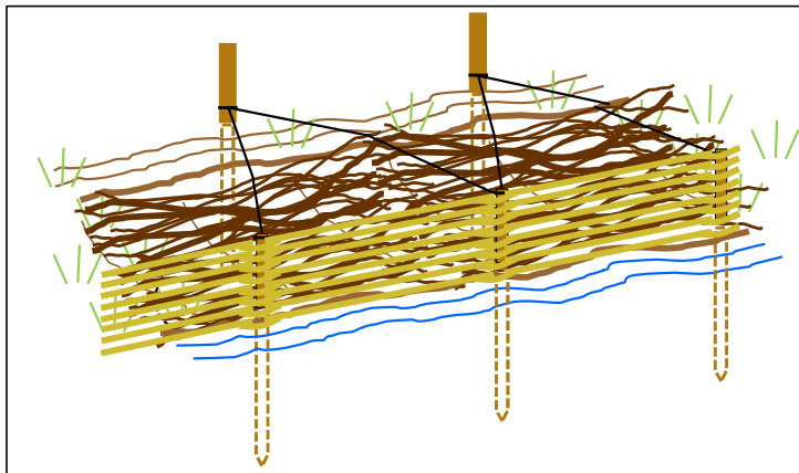
Figure 10c: Securing brash, brash bundles, small trees or large wood to the bank face with wooden stakes or reinforced bar, stainless steel cabling and willow spiling
