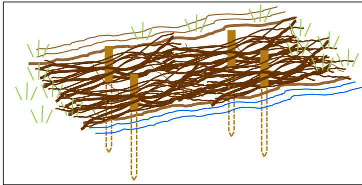
Figure 10a: Securing brash, brash bundles, small trees or large wood to the bank face with wooden stakes or reinforced bar
