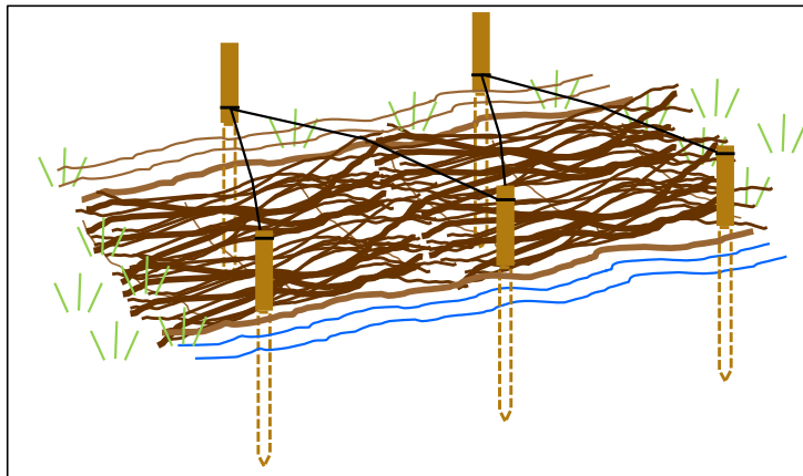
Figure 10b: Securing brash, brash bundles, small trees or large wood to the bank face with wooden stakes or reinforced bar and stainless steel cabling
