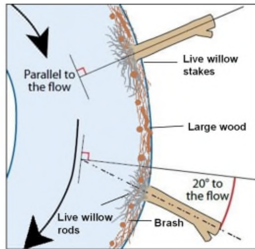
Figure 15: Root wads combined with large wood and brash 3
