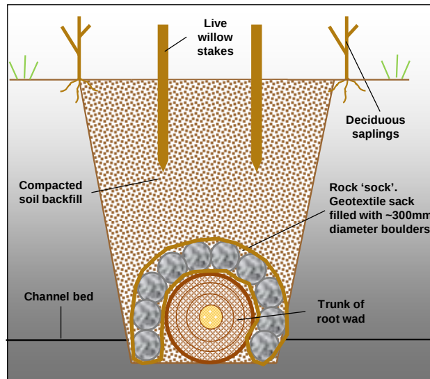
Figure 17c: Cross-section showing root wad stabilisation using a rock roll
